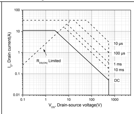
Figure 12, Safe operation area for TO220F T_C=25^\circ\text{C}
