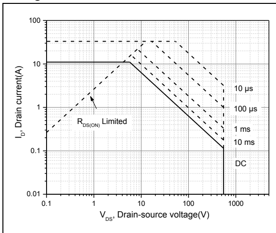
Figure 11, Safe operation area for TO251/TO252/TO220 T_C=25^\circ\text{C}
