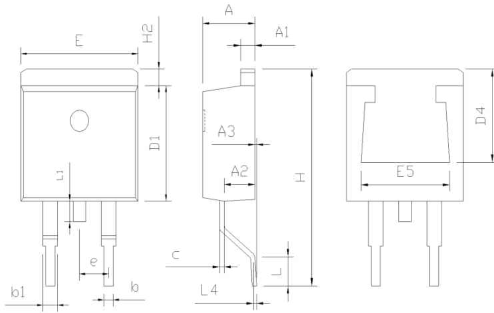
Figure3, TO263 package outline dimension
