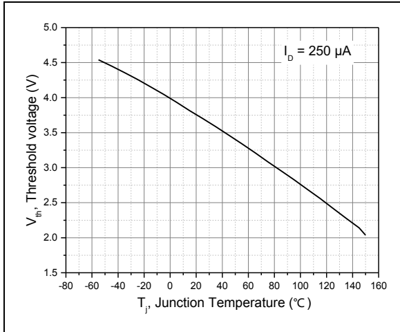
Figure 7, Threshold voltage
